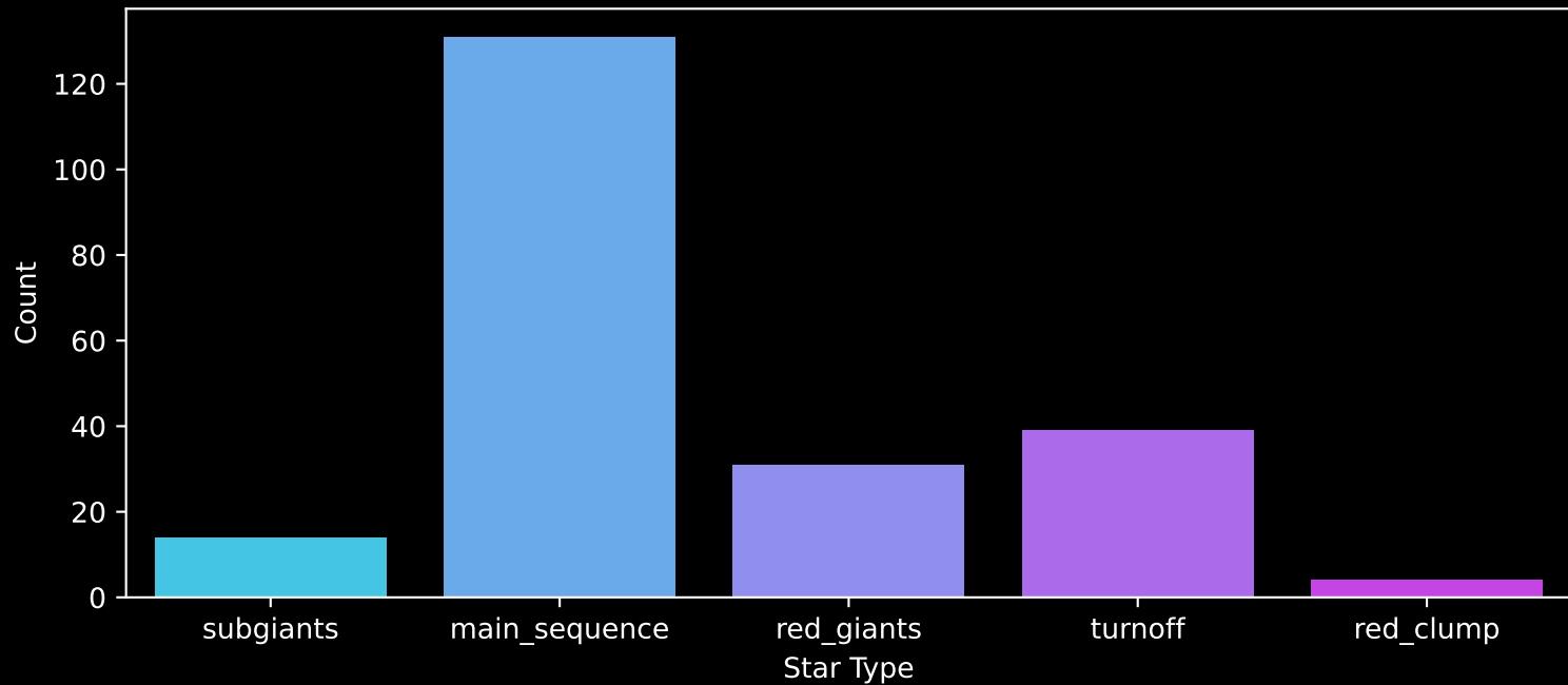
APOGEE DR17 Field: [K2_C5_204+27_btx] Count plot of Star Type
