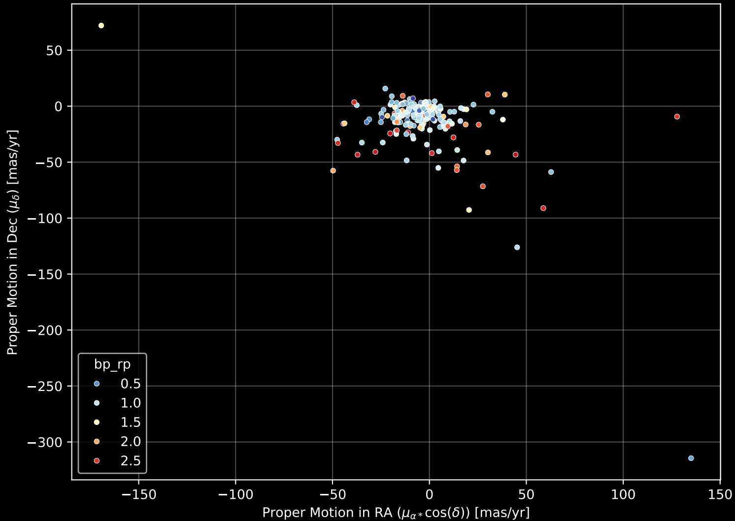
APOGEE DR17 Field: [K2_C5_204+27_btx] Proper Motion Diagram (n= 219)
