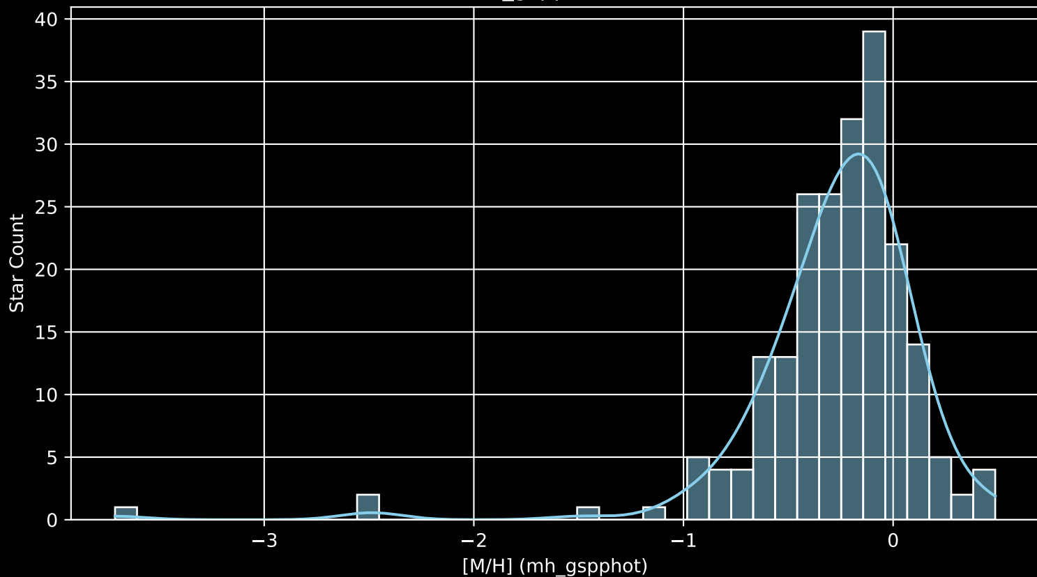
APOGEE DR17 Field: [K2_C5_204+27_btx [M/H] (mh_gspphot) (n= 214)
