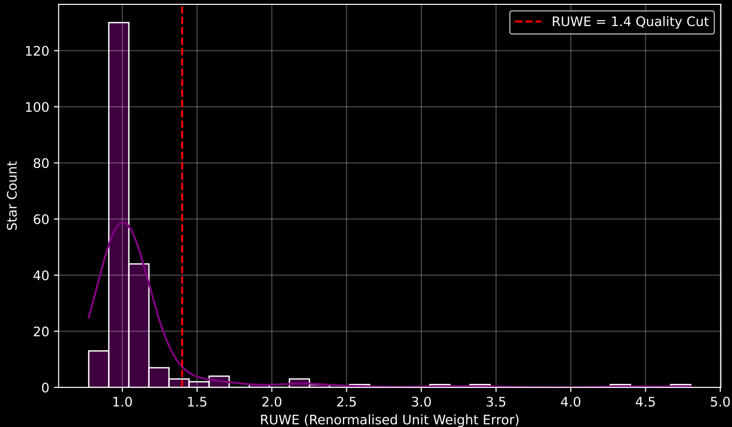
GAPOGEE DR17 Field [K2_C5_204+27_btx] RUWE Distribution (n= 213)
