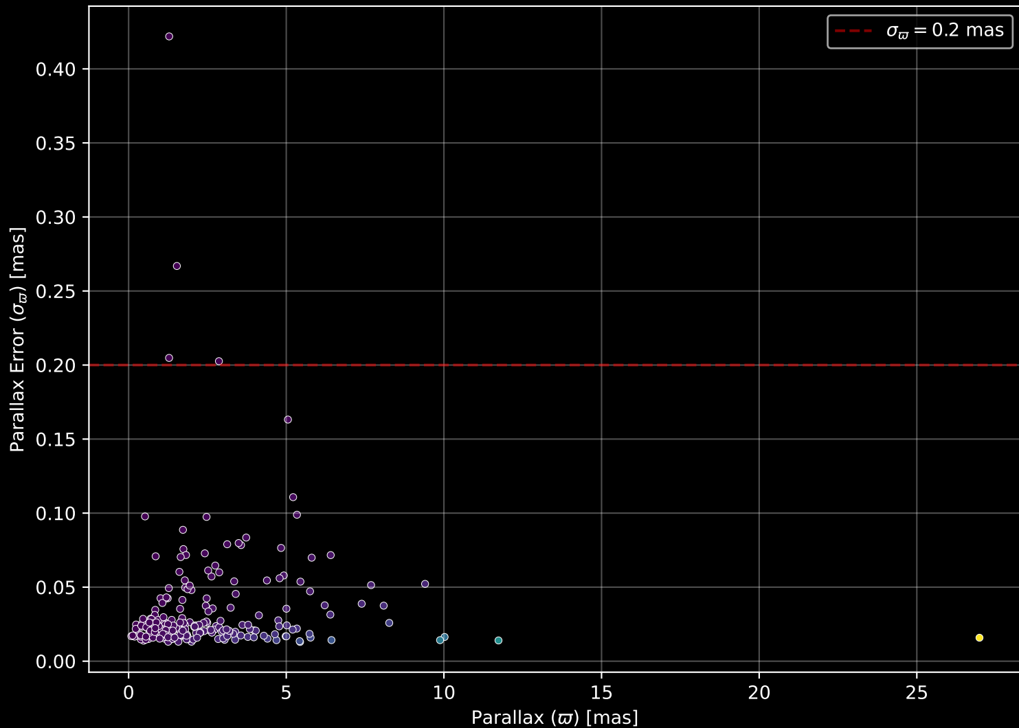
APOGEE DR17 Field: [K2_C5_204+27_btx] Parallax Quality (n= 219)
